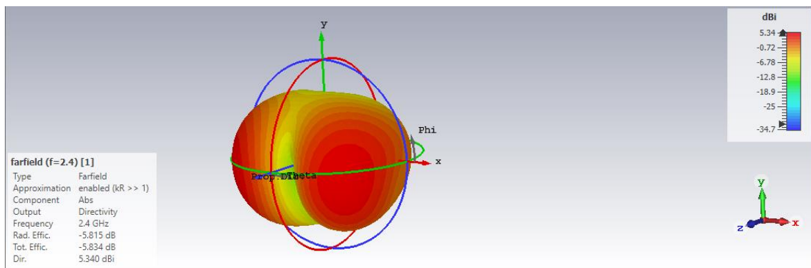
Figure 5. Radiation Pattern at F=2.4 GHz
