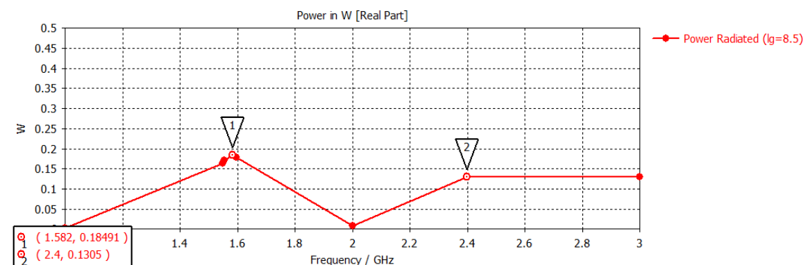
Figure 8. Power Radiated
