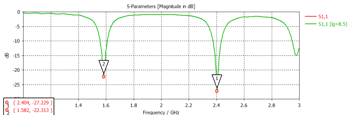
Figure 2. Resonant frequencies
