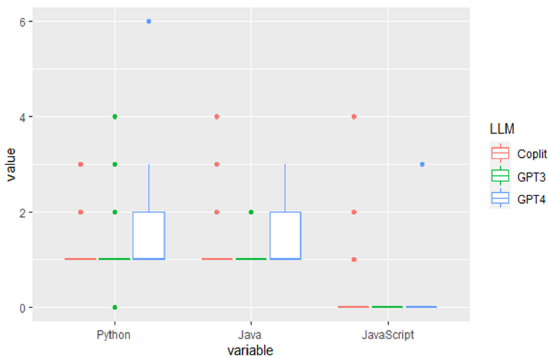
Figure 3 Code Smell Across Models and Languages.
