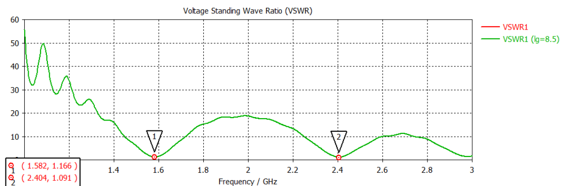
Figure 3. VSWR
