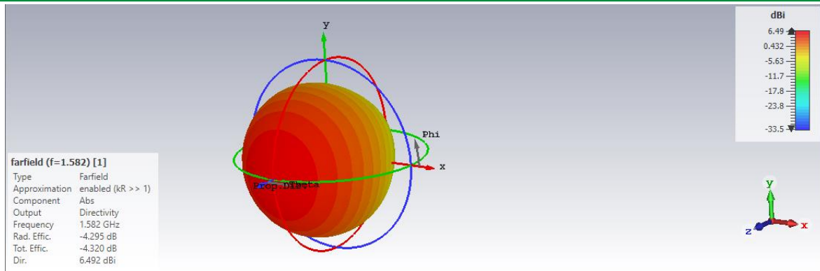
Figure 4. Radiation Pattern at F=1.582
