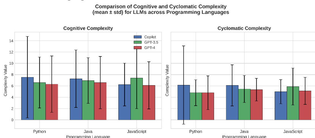
Figure 2 Comparison of Cognitive and Cyclomatic Complexity (mean \pm standard deviation) for code generated by Copilot, GPT-3.5, and GPT-4 across Python, Java, and JavaScript.
