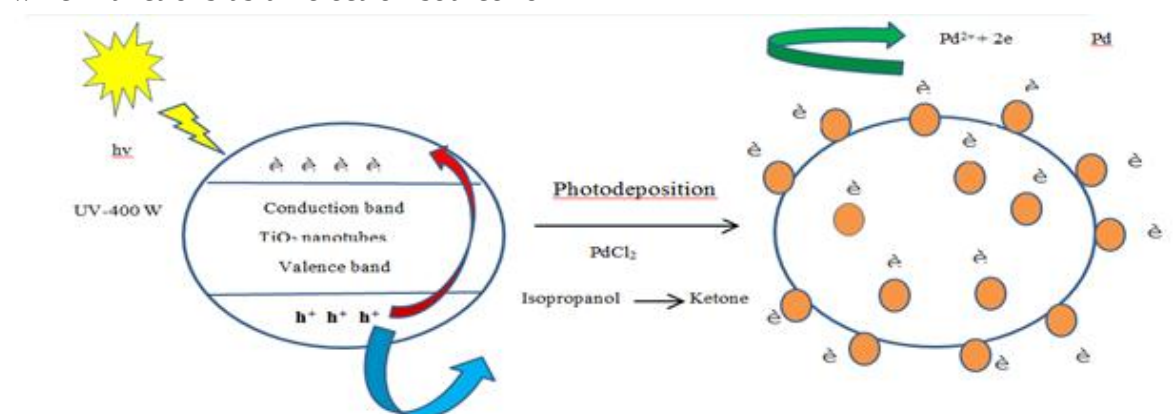
Fig.1: Mechanism of palladium photodeposition (Illustrated drawing for the preparation of Pd-TONTs-N 2 catalyst using UV-400 W lamp photodeposition).
