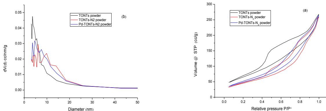
Fig. 6: (a) Adsorption-desorption isotherm of TONTs powder, TONTs-N 2 powder and Pd-TONTs-N 2 powder (b) the average pore diameter, determined through the Barrett-Joyner-Halenda (BJH) method by means of the adsorption isotherm.
