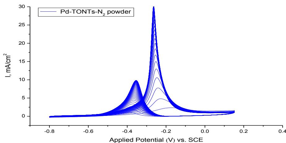
Fig. 12: CV of 3\mu\text{l} Pd-TONTs-N 2 powder, from 1 cycle to 50 cycles loaded on Au working electrode as baseline, all in (2M KOH+1M methanol) at a scan rate was 50 mV/s by current density.
